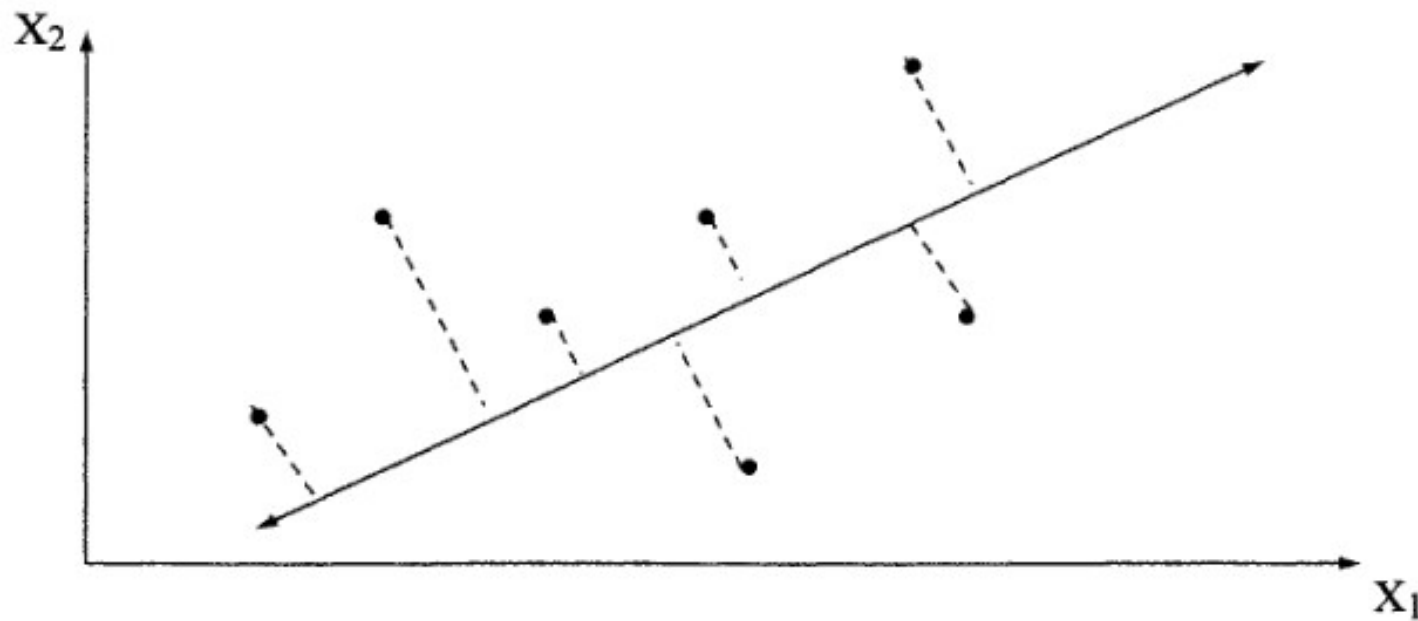
FIGURE 3.2 The first principal component is an axis in the direction of maximum variance
